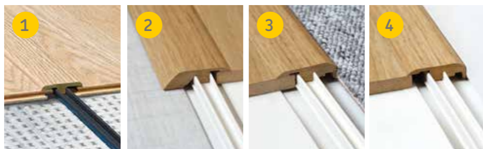
Expansion Profile 2150 x 40 x 13mm Adaptor Profile 2150 x 48 x 13mm Transition Profile 2150 x 40 x 13mm Edge Profile 2150 x 40 x 13mm
